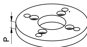
Adapterplatte (ADP)
